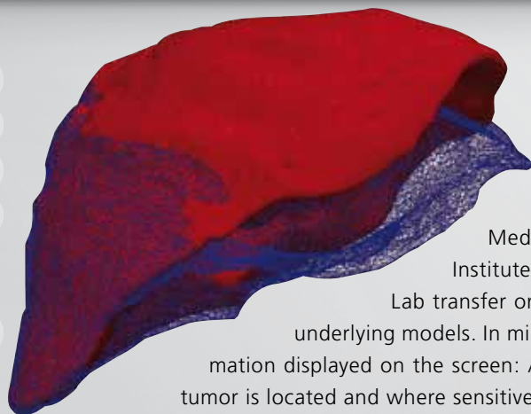
Organmodell Leber
